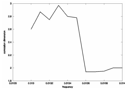
Figure3: Correlation dimension vs. pump frequency
